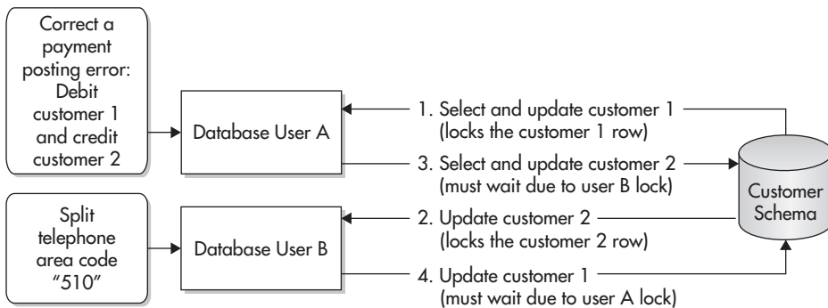
Figure 11-2 The deadlock
